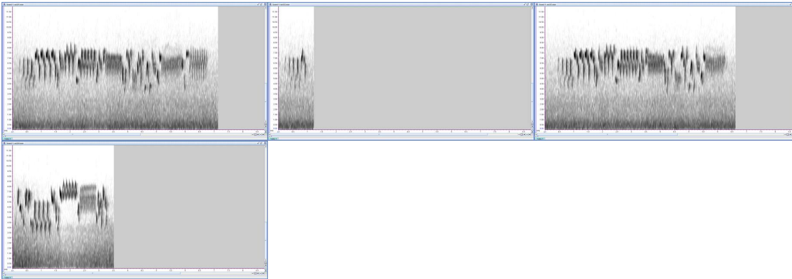
Sonograms from recordings of singing Pacific wren in Rocky Mountain National Park.
